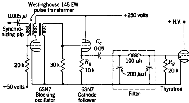
FIG. 8-54.—Typical hydrogen-thyatron trigger generator.
